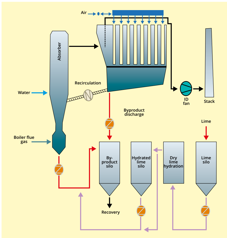
Above: Figure 1. The CFB dry desulphurisation process (with fabric filter). Source: Sumitomo SHI FW
